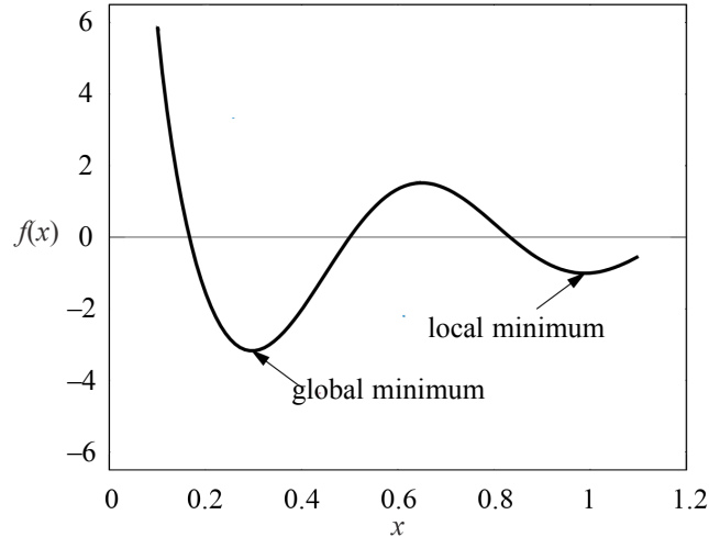
Figure 2: A local and a global minima of a function.
